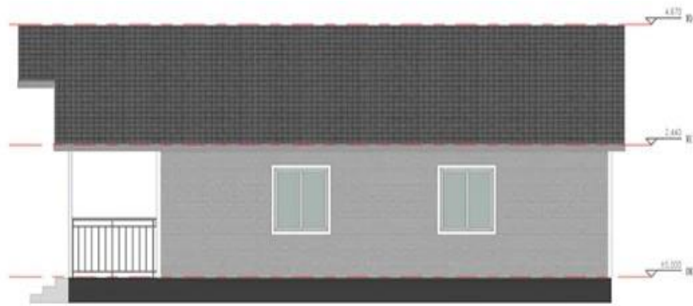
EAST ELEVATION
